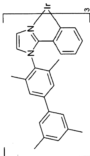
Compound 2
