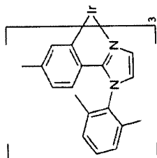
Compound I
