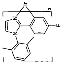
Compound G
