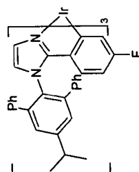
Compound K
