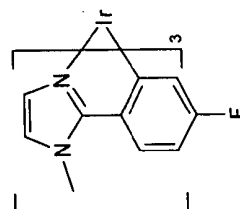
Compound L
