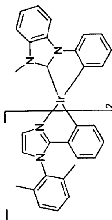
Compound 3
