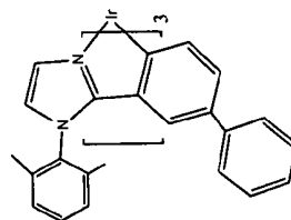
Compound J
