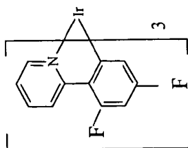
Compound F
