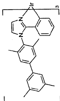
Compound H
